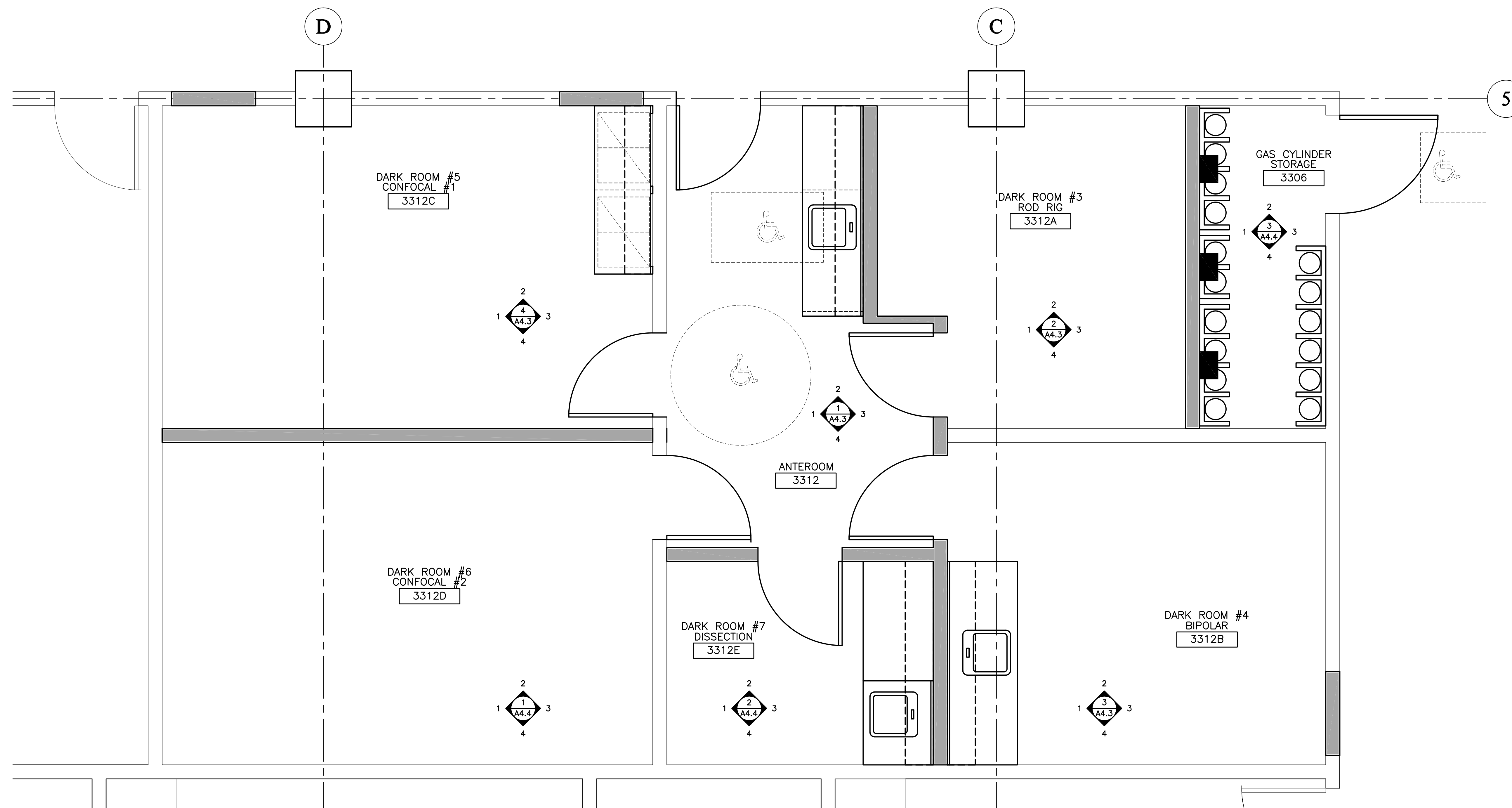
1 CASEWORK LAYOUT ROOMS: 3306, 3312, 3312A, 3312B, 3312C, 3312D, 3312E
